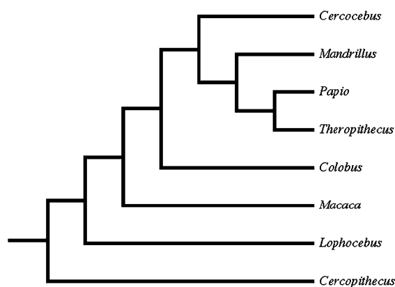
Fig. 3. Most parsimonious cladogram derived from mixed-sex low-to-moderate-strain characters.
