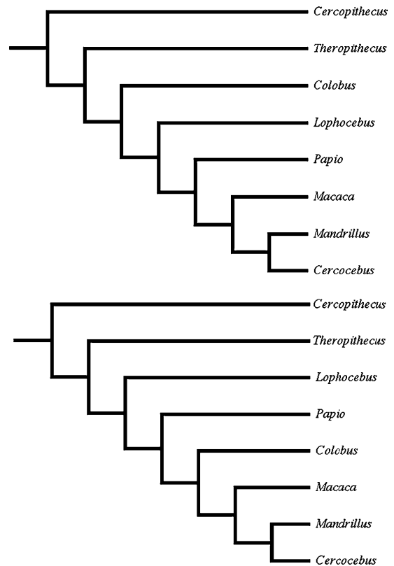
Fig. 7. Most parsimonious cladograms derived from mixed-sex dental characters that remain significantly correlated with the geometric mean after size-correction.
