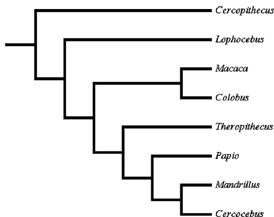
Fig. 4. Most parsimonious cladogram derived from mixed-sex dental characters.
