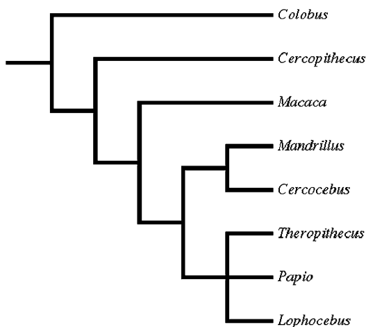
Fig. 1. Consensus molecular phylogeny for the taxa used in this study.
