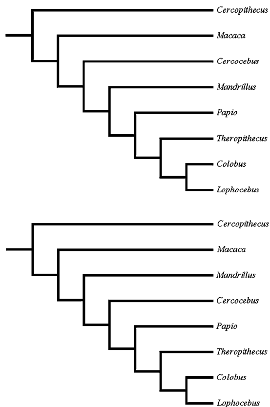
Fig. 5. Most parsimonious cladograms derived from mixed-sex high-strain characters after removal of characters that remain significantly correlated with the geometric mean after size-correction.
