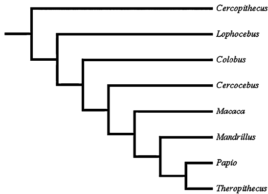
Fig. 6. Most parsimonious cladogram derived from mixed-sex low-to-moderate-strain characters after removal of characters that remain significantly correlated with the geometric mean after size-correction.
