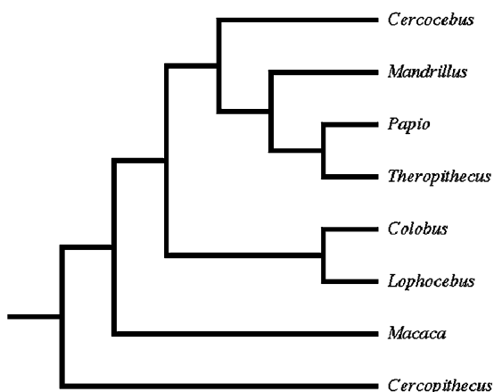
Fig. 2. Most parsimonious cladograms derived from mixed-sex high-strain characters.
