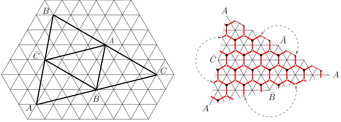
Figure 2: An example of Construction 4.1.
