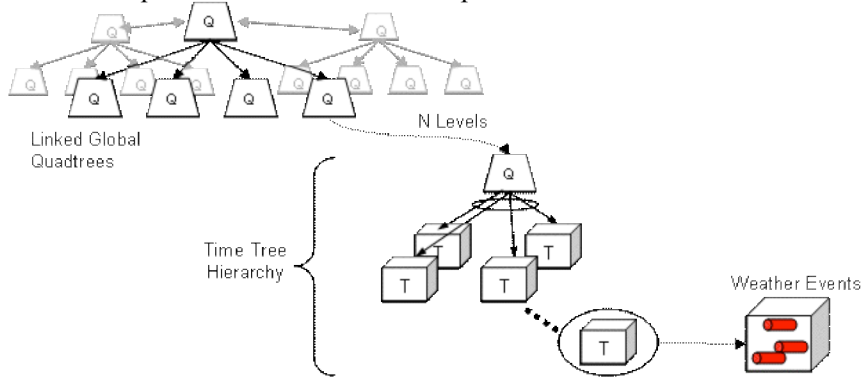
Figure 4-2. Data-adapted global quadtree for time-dependent volume data
