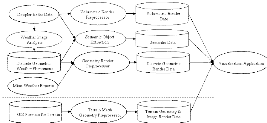
Figure 4-3. High level dataflow diagram of system.
